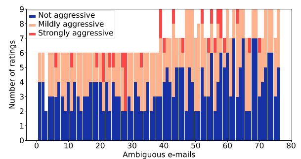
Fig. 4. Overview of how many annotators had chosen which overall label (i.e., aggressive or non-aggressive), separately for each of the 76 ambiguous e-mails (i.e., the e-mails for which the number of annotators who had selected targets Human or Technical for an e-mail is greater than the number of annotators who had labeled this e-mail as aggressive).
