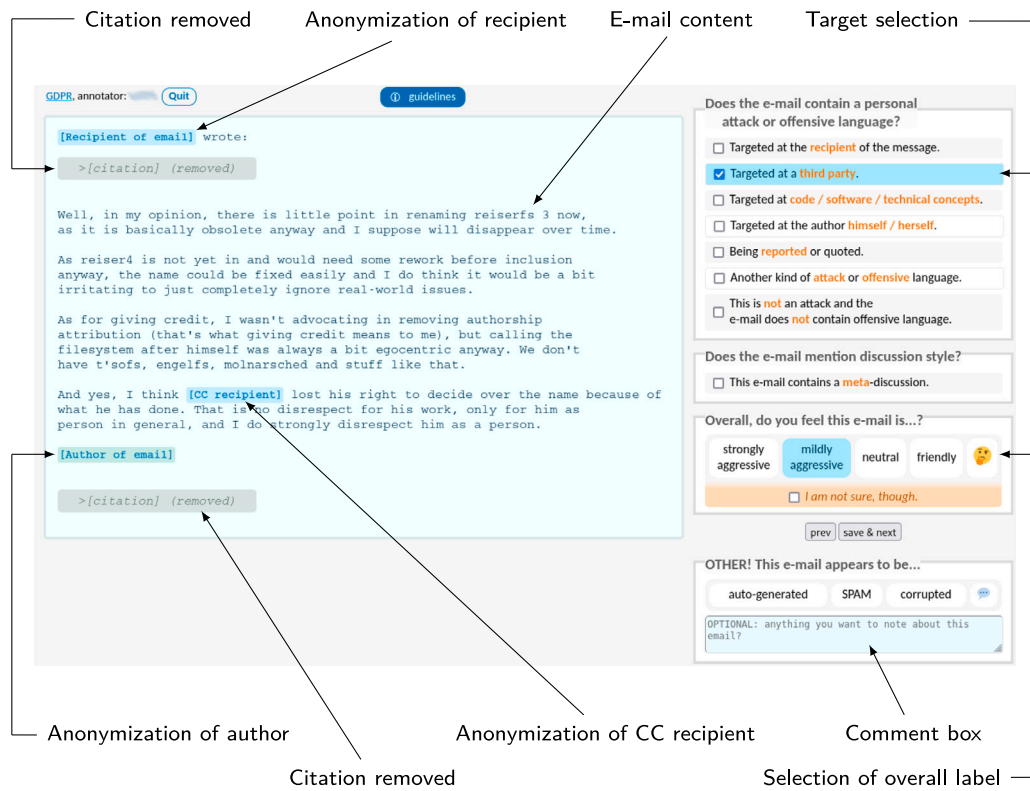
Fig. 1. Example screenshot of our annotation tool (with additional explanations surrounding the screenshot).
