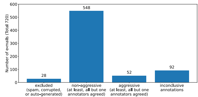
Fig. 3. General overview of the results of our annotation study on 720 e-mails from the LKML (excluding unsure annotations, that is, annotations that have been marked as “I am not sure” by the annotator).
