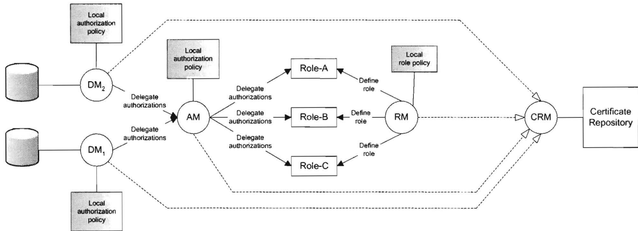
Figure 1: Authorization modules
