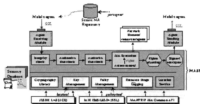
Figure 5: Mobile Agent Security Facility (MASF) Architecture
