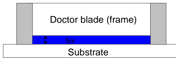
Figure 2. Wet layer thickness control by the gap between the frame and the blade.
